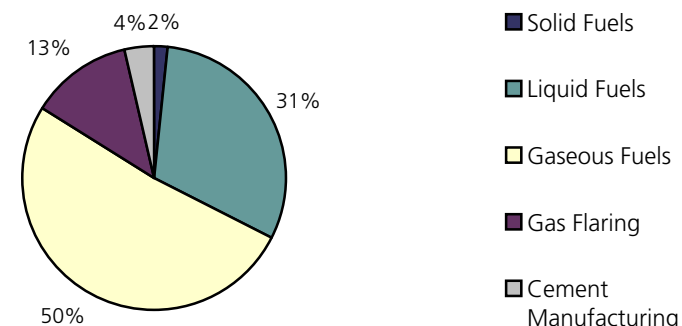
CO 2 Emissions by Source, Algeria, 1998
