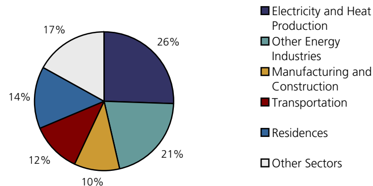
CO 2 Emissions by Sector, Algeria, 1999
