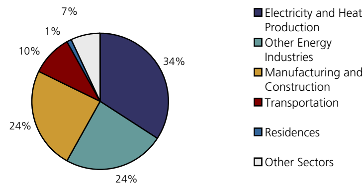
CO 2 Emissions by Sector, Bahrain, 1999
