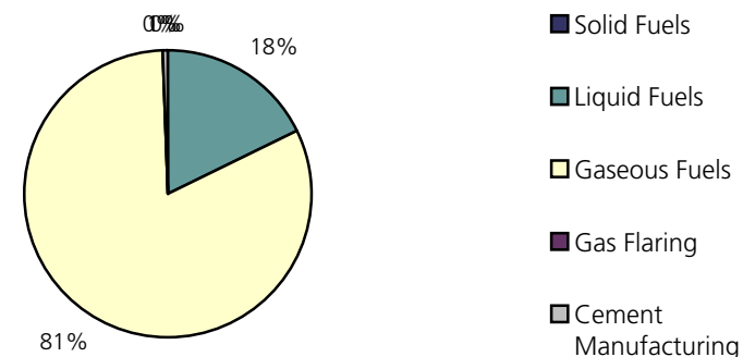
CO 2 Emissions by Source, Bahrain, 1998
