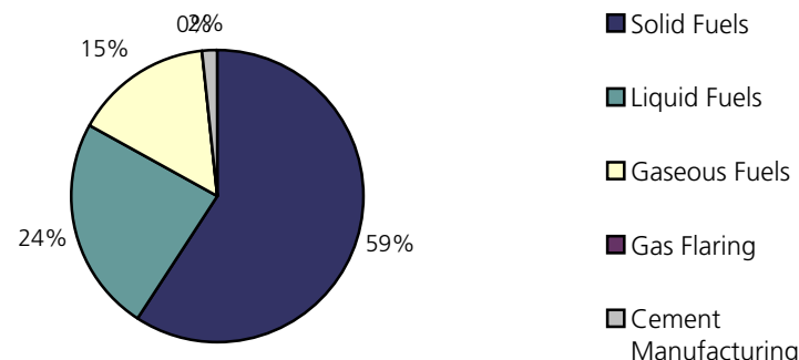
CO 2 Emissions by Source, Bulgaria, 1998
