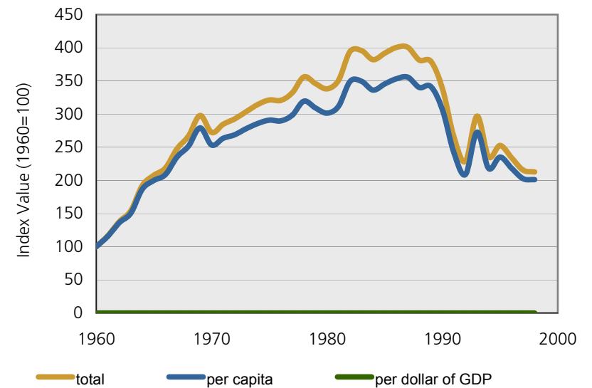
CO2 emissions: Relative Trends, Bulgaria, 1960-1998
