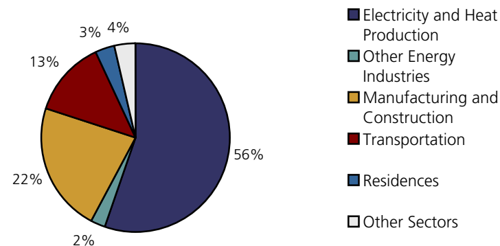
CO 2 Emissions by Sector, Bulgaria, 1999
