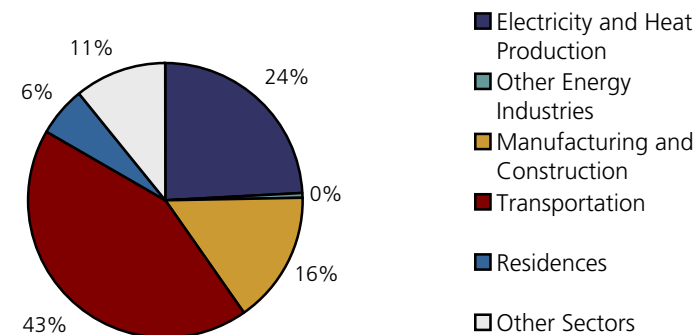
CO 2 Emissions by Sector, Guatemala, 1999
