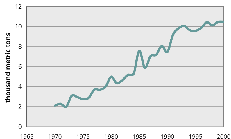
Average Annual Capture of Marine Fish, Bahamas
