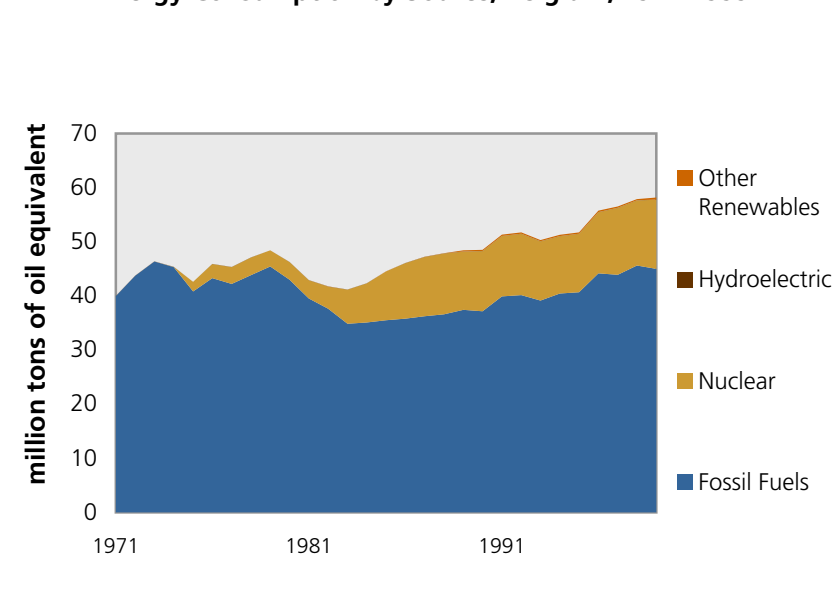
Energy Consumption by Source, Belgium, 1971-1999
