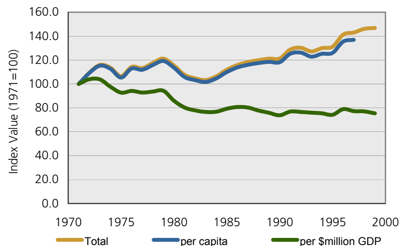
Energy Consumption: Relative trends, Belgium, 1971-1999
