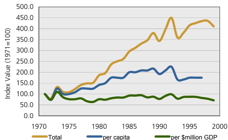
Energy Consumption: Relative trends, Yemen, 1971-1999
