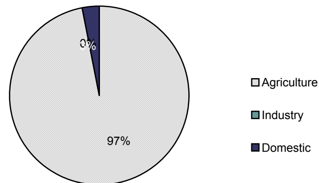
Surface Water Withdrawals by Sector, Somalia, 1987
